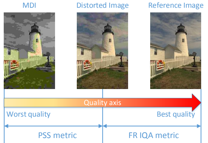
Fig. 1. A compare of the proposed PSS metric and FR IQA metric. FR IQA metric calculates the “distance” between the distorted and reference image, while PSS calculates the “distance” between the distorted and most distorted image.
