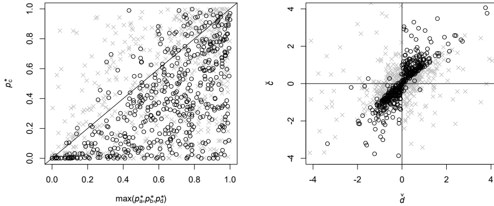
Figure 8: Numerical exploration for the LAD- Z framework: black circles represent datasets with \check{\rho}_{bd} > 0 , and grey crossings represent datasets with \check{\rho}_{bd} \leq 0 .
