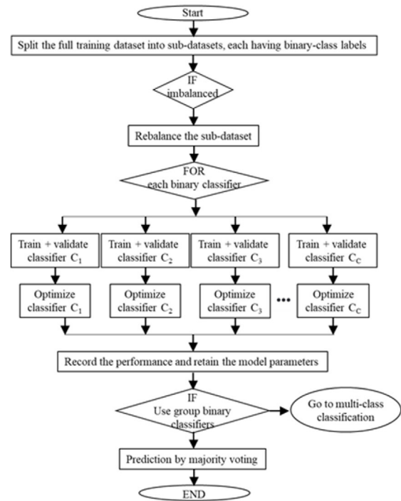
Fig. 3a. The workflow of Group-of-Single-Class prediction methodology – Part one, when MCC is not needed.
