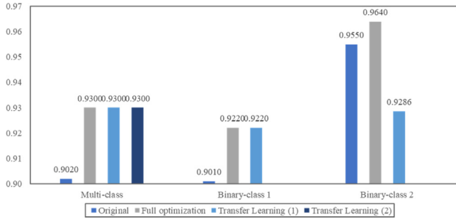
Fig. 8c. ROC comparison of models by Rule-based Model – PART.
