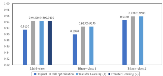
Fig. 8a. ROC comparison of models by Decision Tree – J48.
