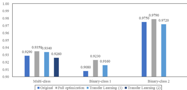
Fig. 8e. ROC comparison of models by Black-box Model – Neural Network.
