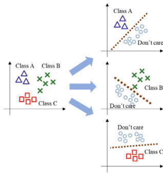
Fig. 1. Multiple one-versus-all binary-class classifiers.
