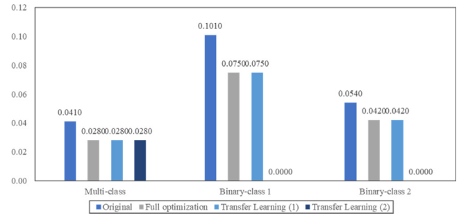
Fig. 9a. FP comparison of models by Decision Tree – J48.
