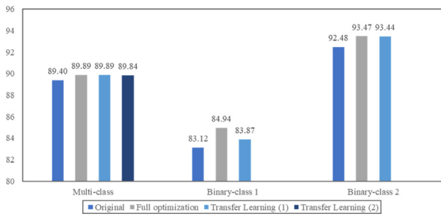
Fig. 6d. Accuracy comparison of models by Rule-based Model – JRip.
