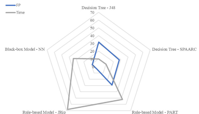
Fig. 12. Radar chart of performance indicators comparison of False Positive Rate and Time cost.
