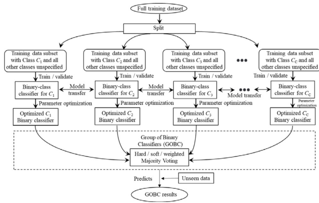
Fig. 2b. The framework of Group-of-Single-Class prediction methodology.
