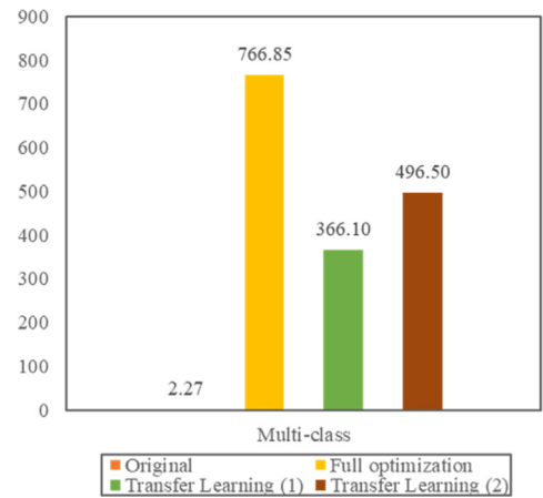
Fig. 10c. Time comparison of models by Rule-based Model – PART.
