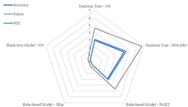
Fig. 11. Radar chart of performance indicators comparison of Accuracy, Kappa and ROC.
