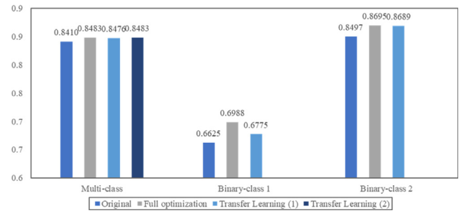
Fig. 7d. Kappa comparison of models by Rule-based Model – JRip.
